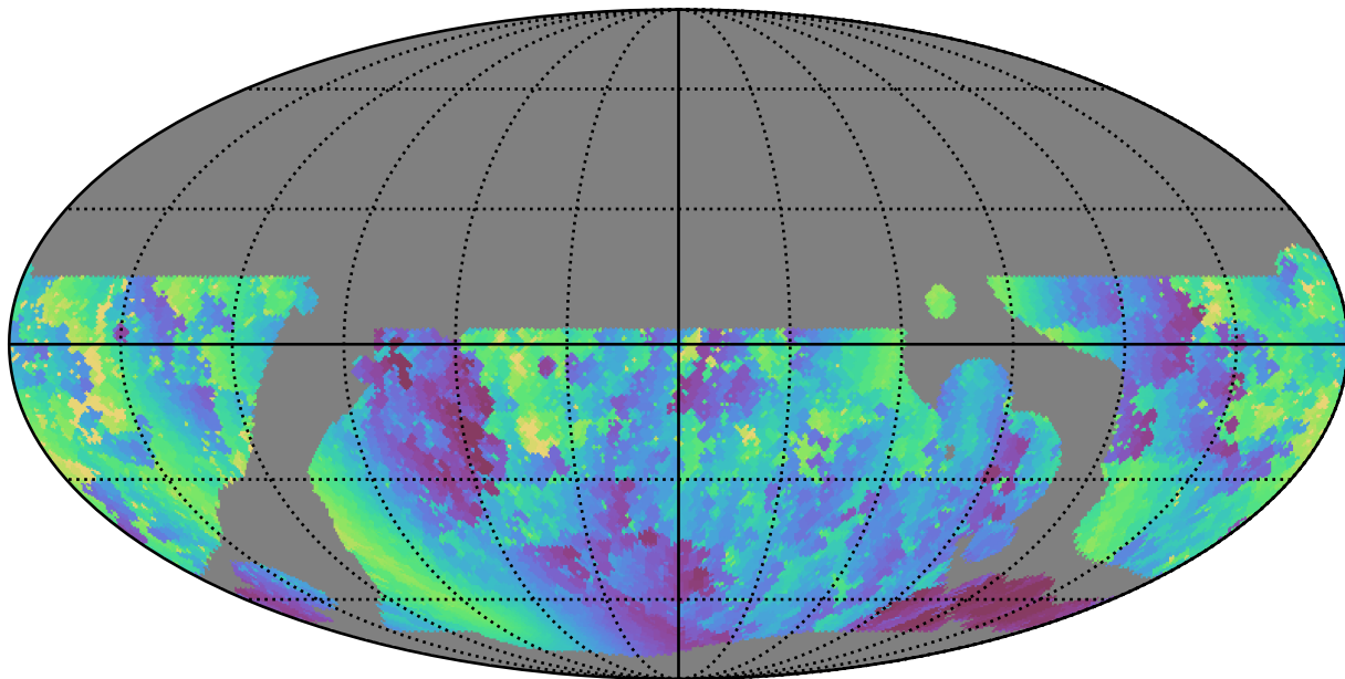
weather_cloudso0v3.5_10yrs WFD g band: Min solarElong
