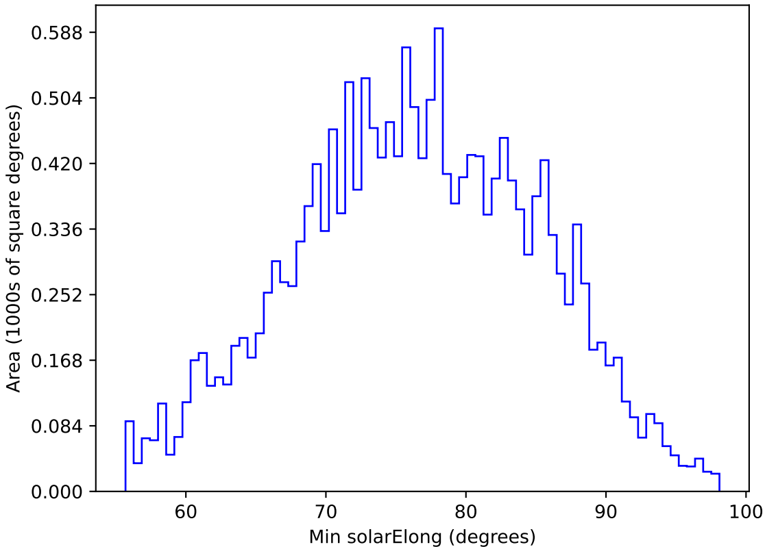
weather_cloudso0v3.5_10yrs WFD g band: Min solarElong
