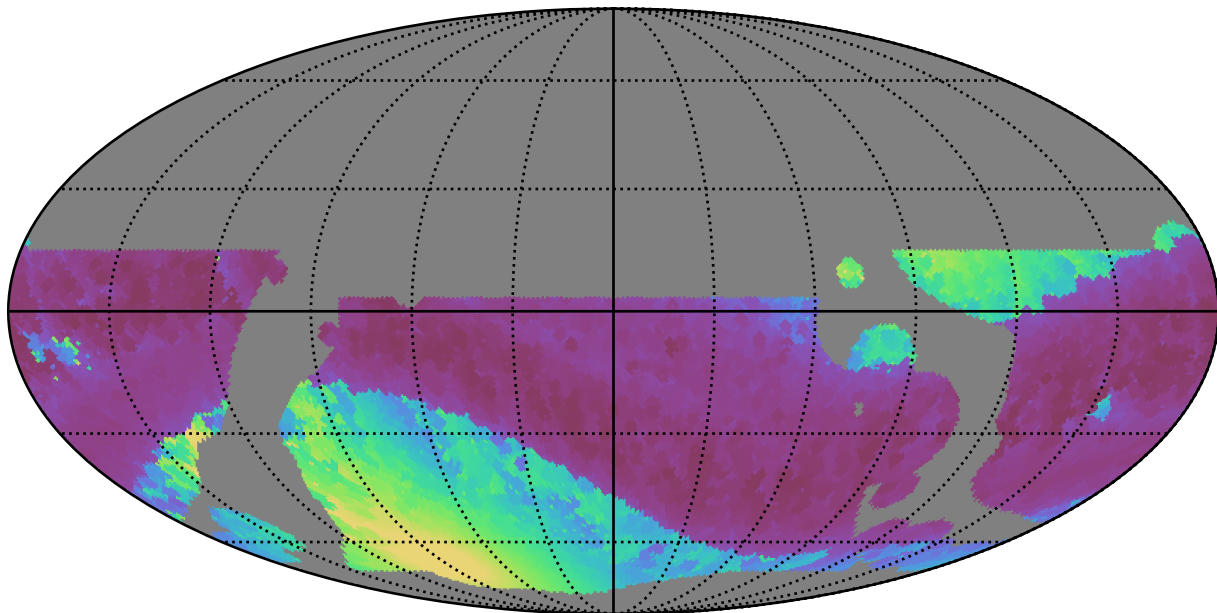
weather_cloudso0v3.5_10yrs WFD all bands: Min solarElong
