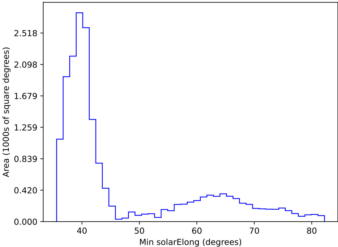
weather_cloudso0v3.5_10yrs WFD all bands: Min solarElong
