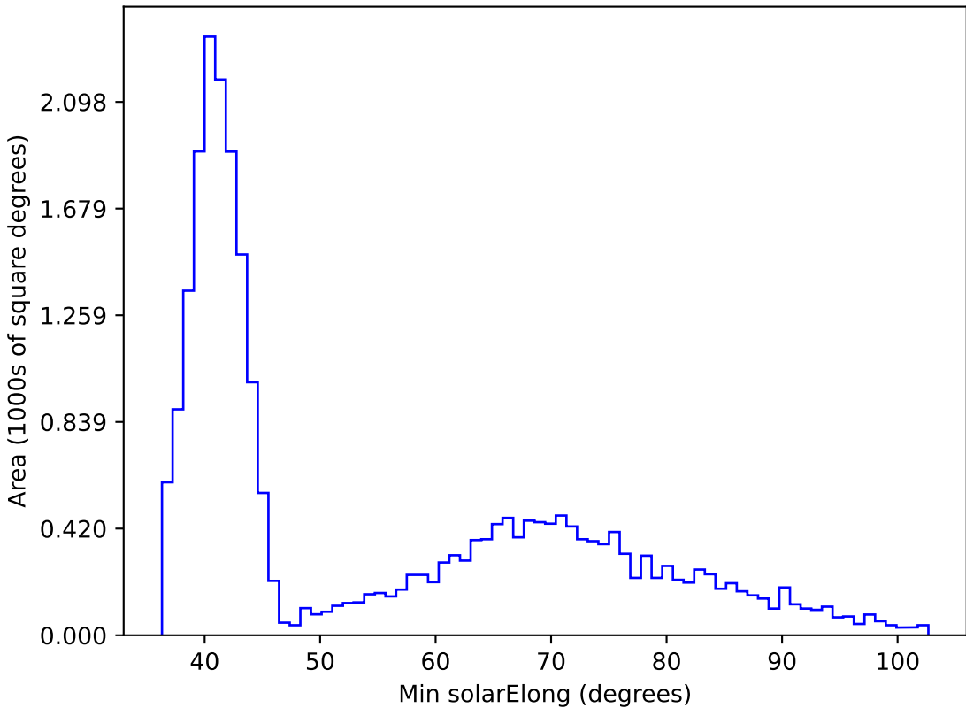
weather_cloudso0v3.5_10yrs All sky z band: Min solarElong
