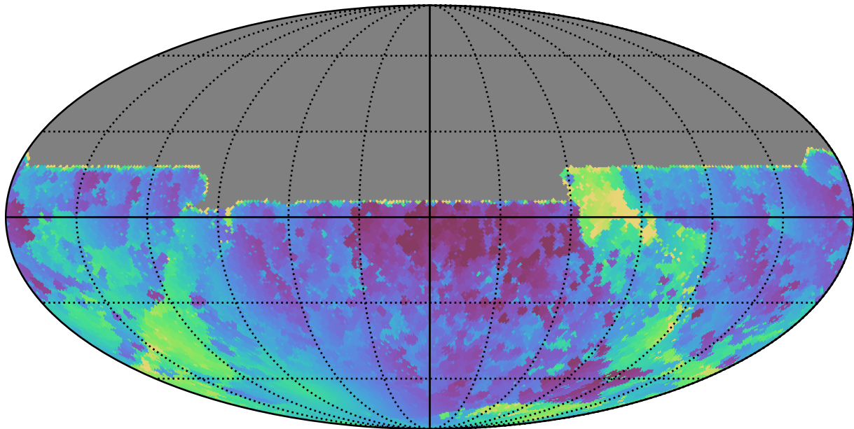
weather_cloudso0v3.5_10yrs All sky y band: Min solarElong
