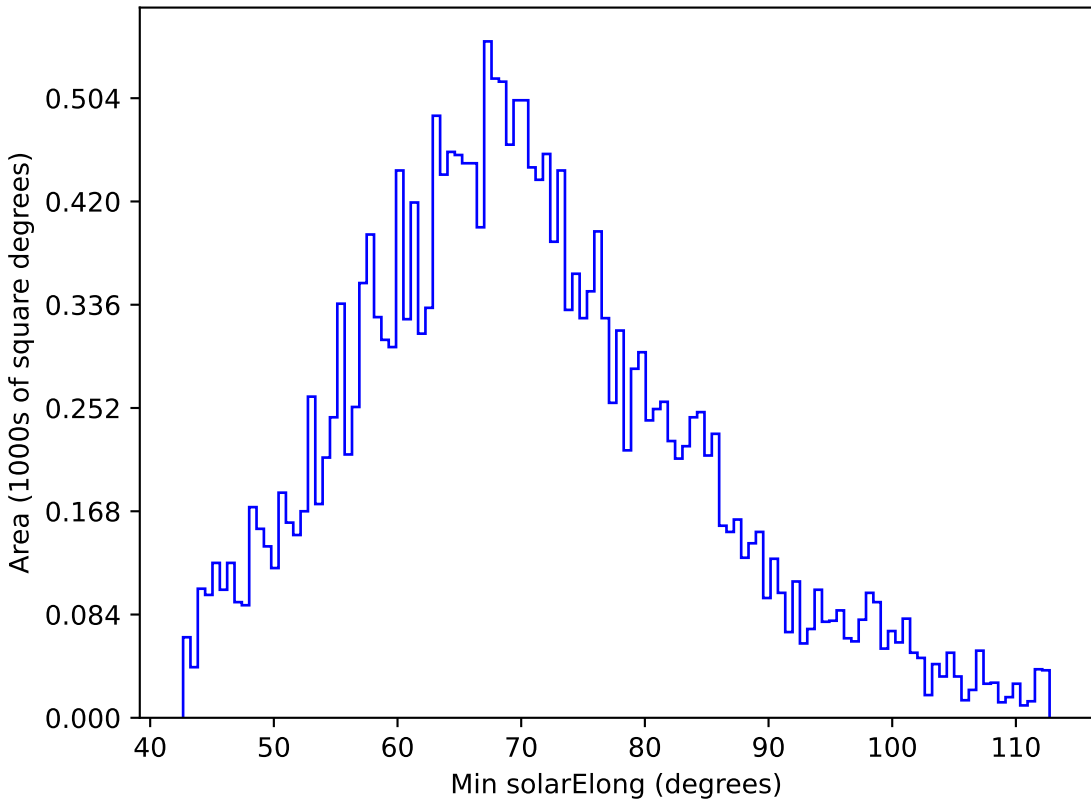
weather_cloudso0v3.5_10yrs All sky y band: Min solarElong
