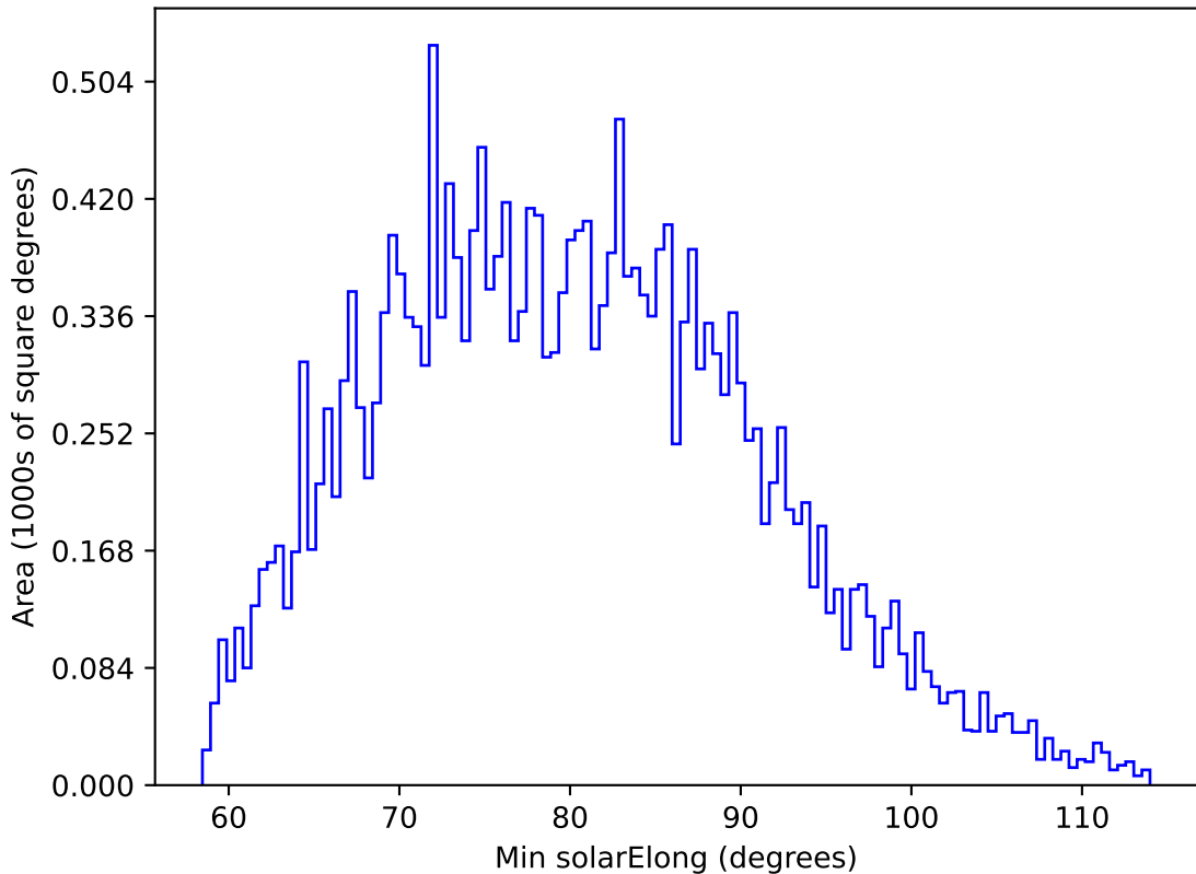
weather_cloudso0v3.5_10yrs All sky u band: Min solarElong
