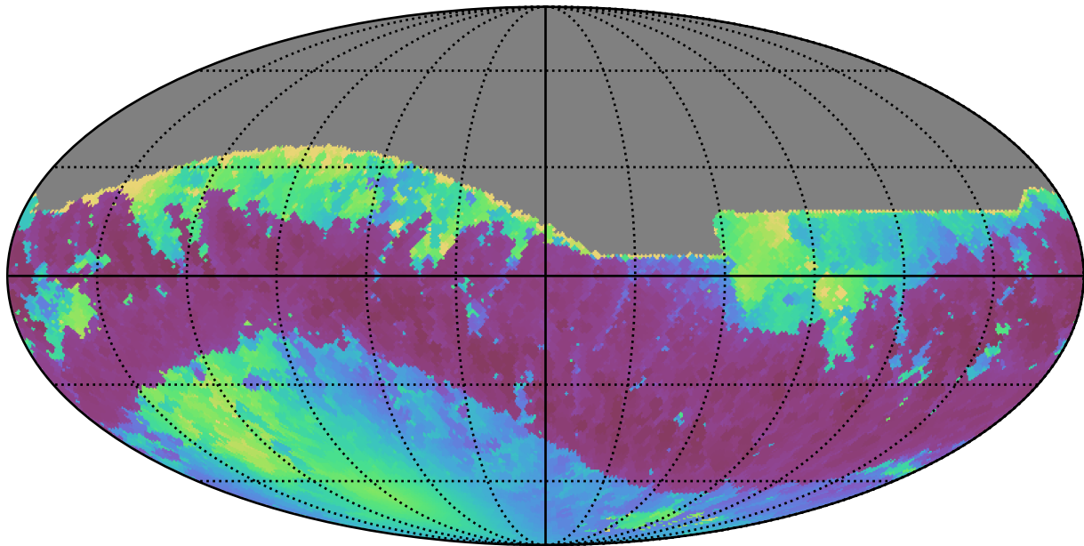
weather_cloudso0v3.5_10yrs All sky r band: Min solarElong
