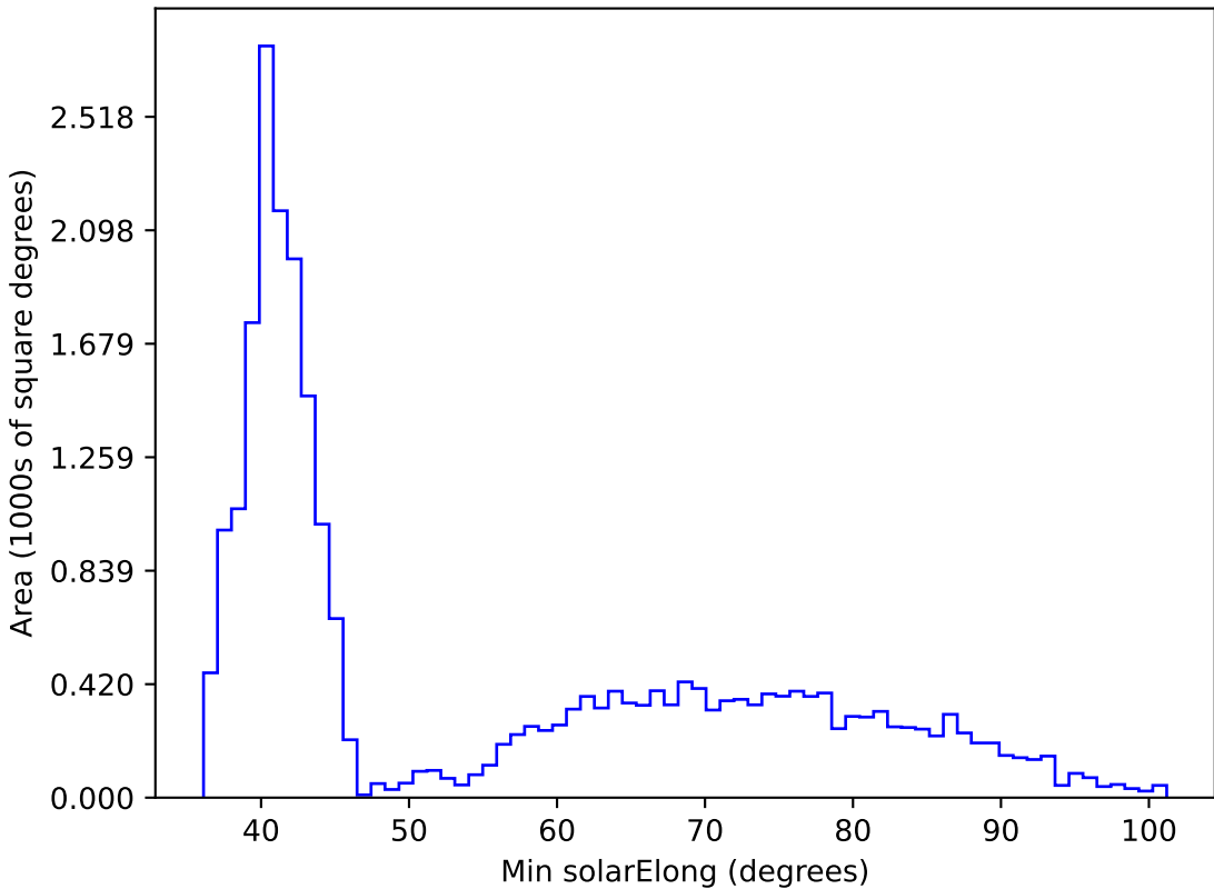
weather_cloudso0v3.5_10yrs All sky r band: Min solarElong
