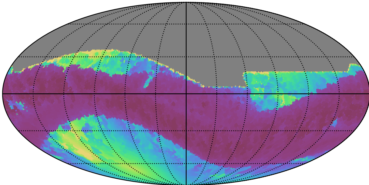
weather_cloudso0v3.5_10yrs All sky all bands: Min solarElong
