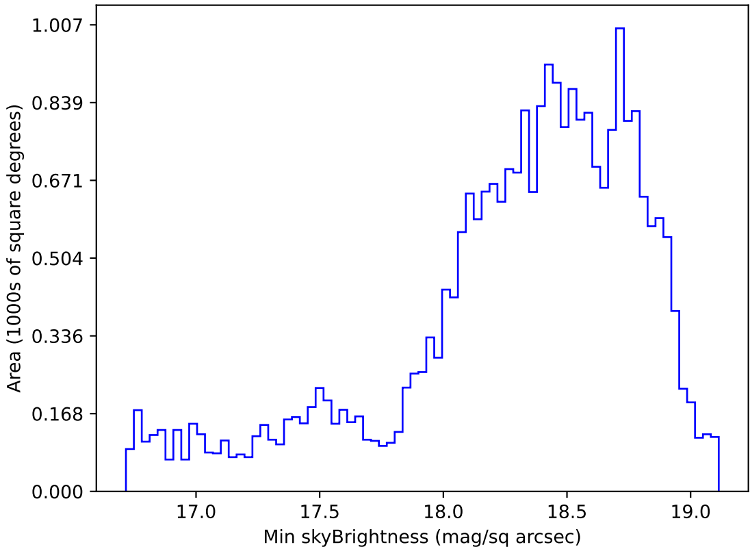
weather_cloudso0v3.5_10yrs Yr 1 z band: Min skyBrightness
