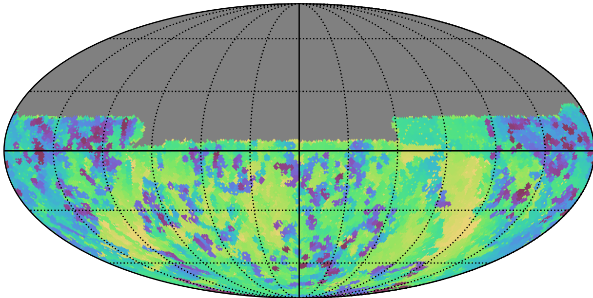
weather_cloudso0v3.5_10yrs Yr 1 y band: Min skyBrightness
