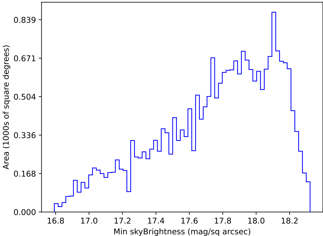
weather_cloudso0v3.5_10yrs Yr 1 y band: Min skyBrightness
