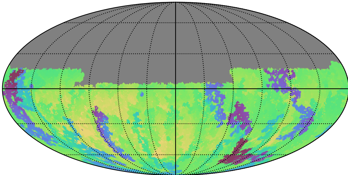
weather_cloudso0v3.5_10yrs Yr 1 u band: Min skyBrightness
