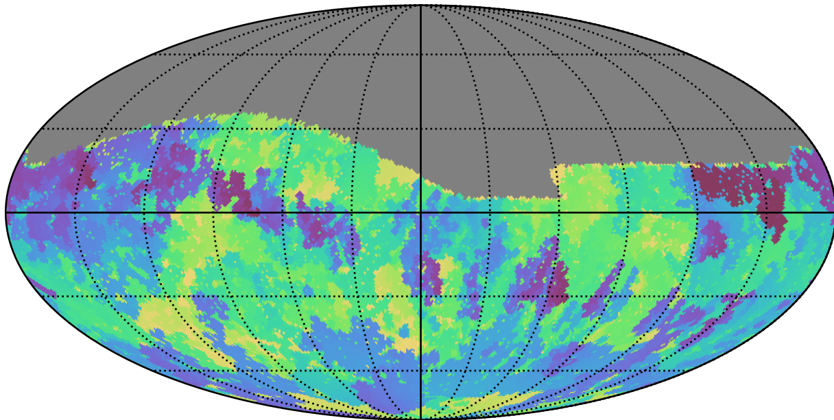
weather_cloudso0v3.5_10yrs Yr 1 r band: Min skyBrightness
