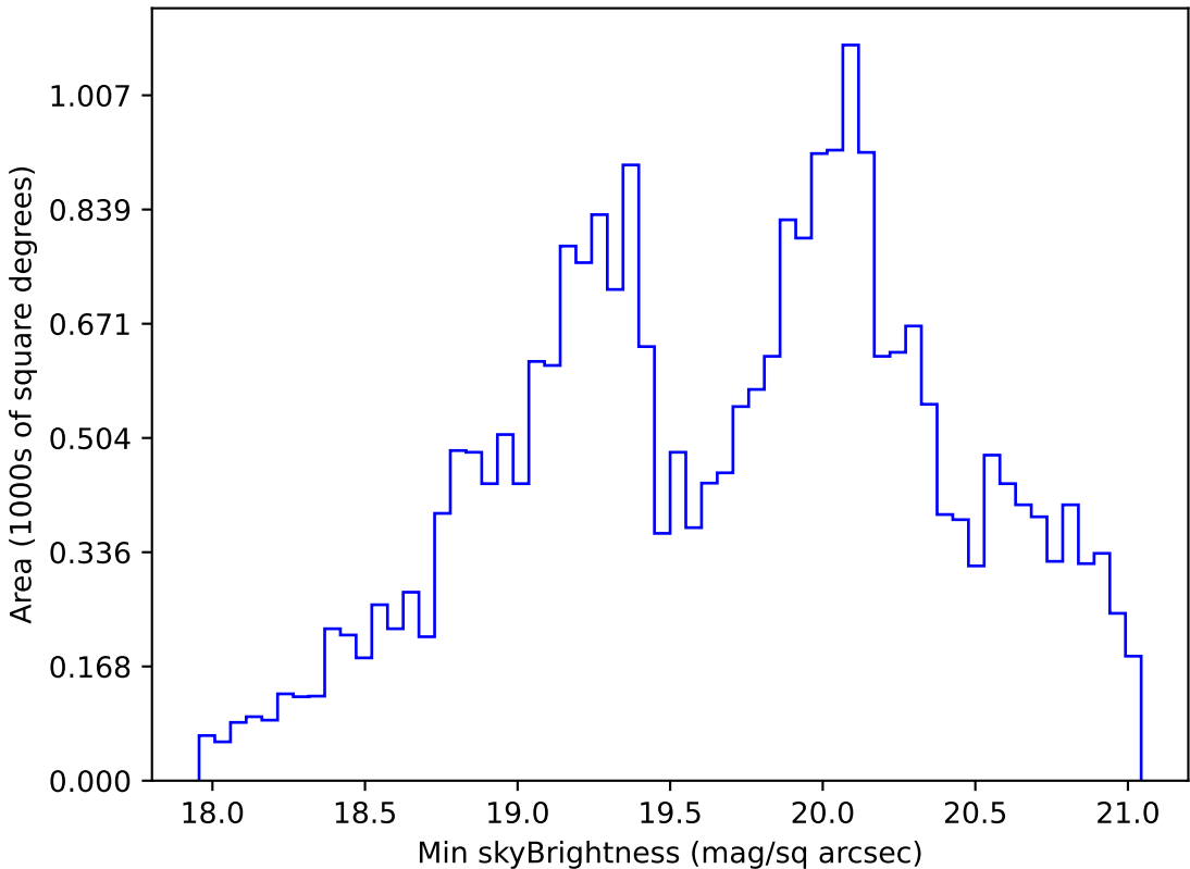
weather_cloudso0v3.5_10yrs Yr 1 r band: Min skyBrightness
