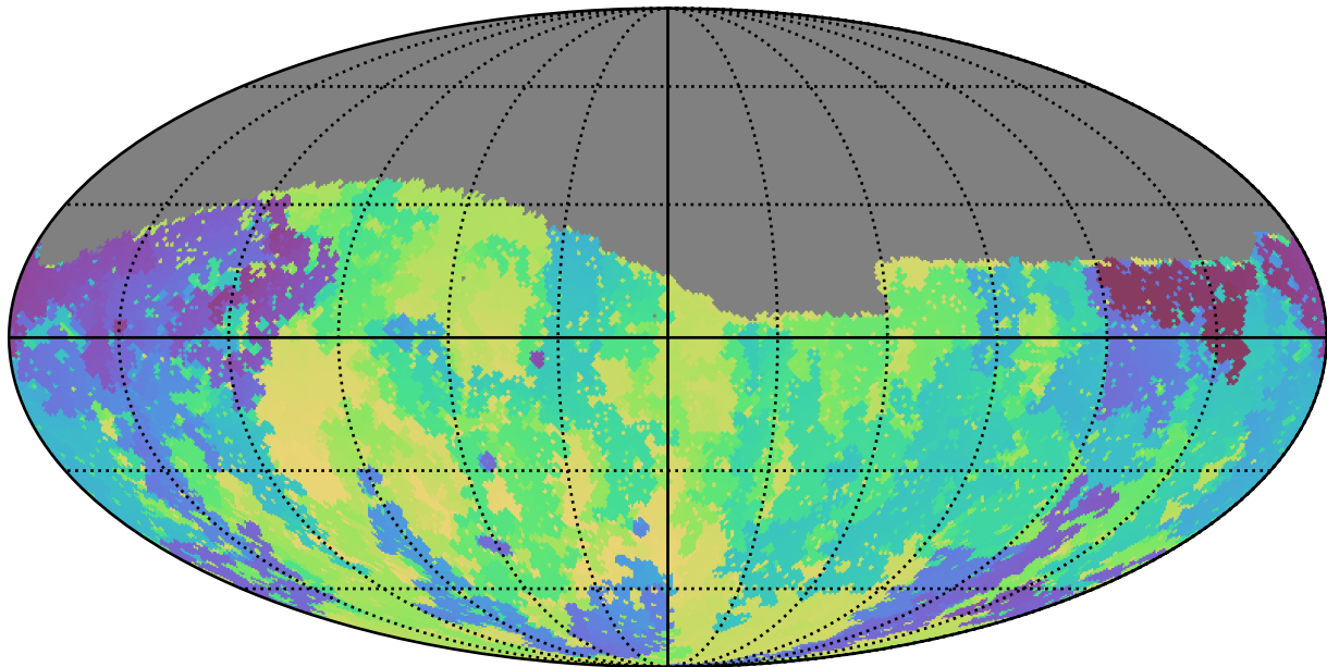
weather_cloudso0v3.5_10yrs Yr 1 g band: Min skyBrightness
