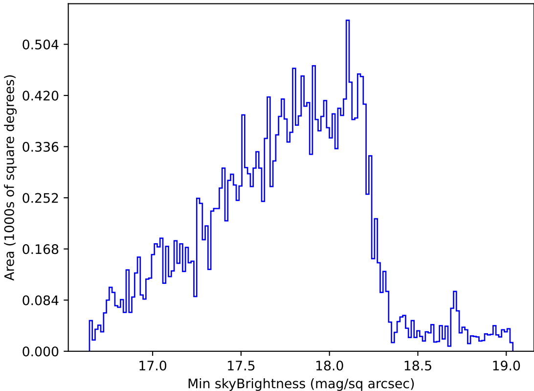
weather_cloudso0v3.5_10yrs Yr 1 all bands: Min skyBrightness
