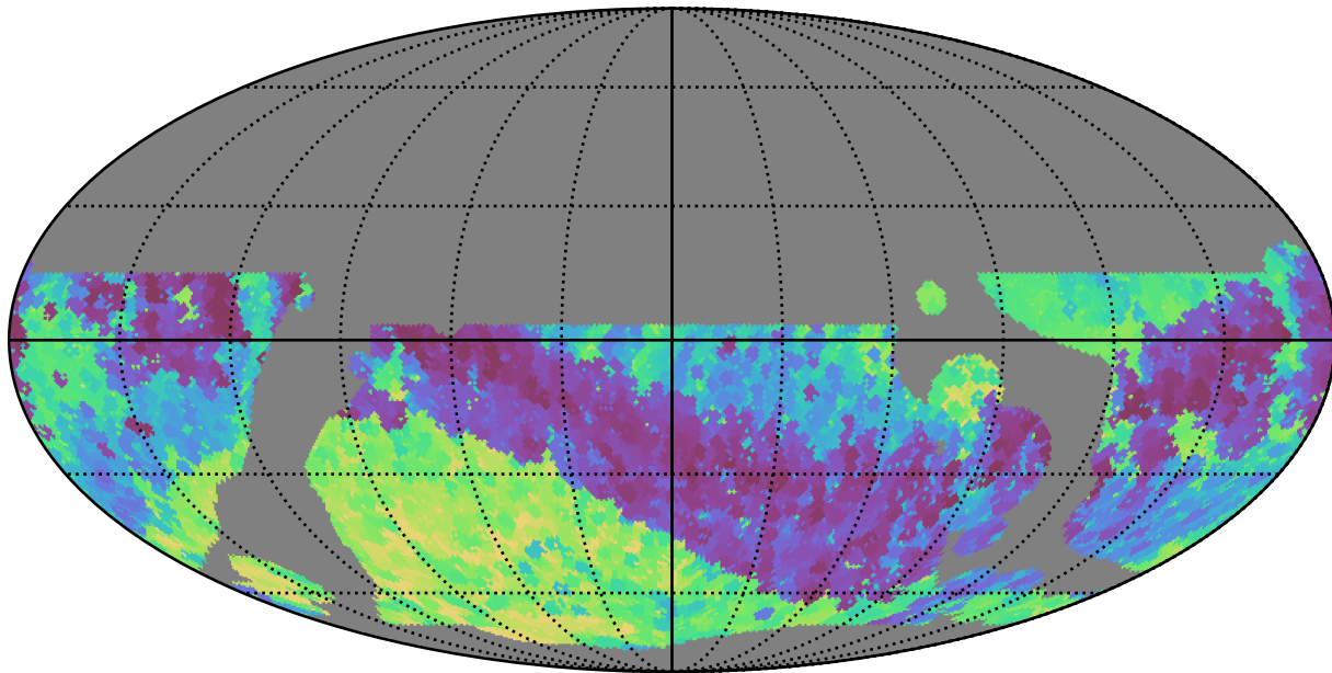
weather_cloudso0v3.5_10yrs WFD z band: Min skyBrightness
