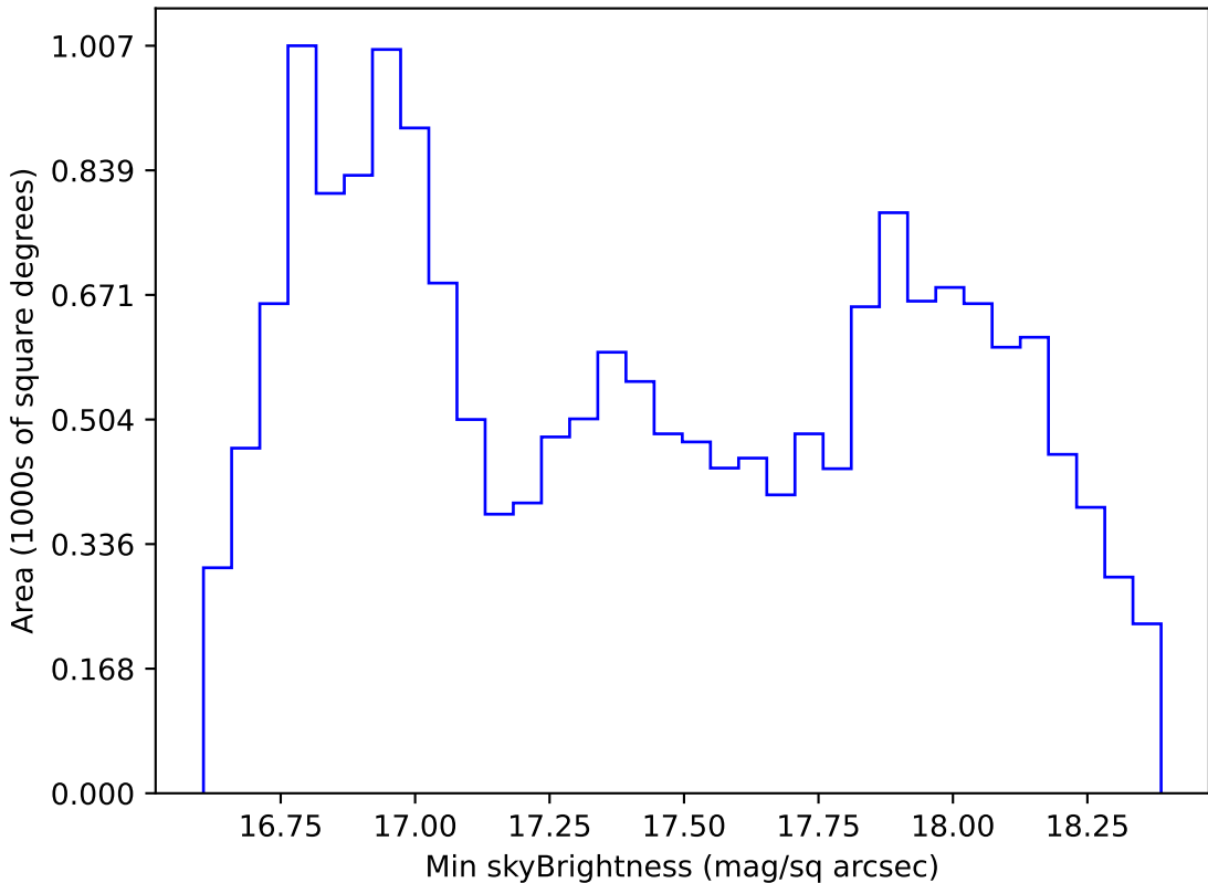
weather_cloudso0v3.5_10yrs WFD z band: Min skyBrightness
