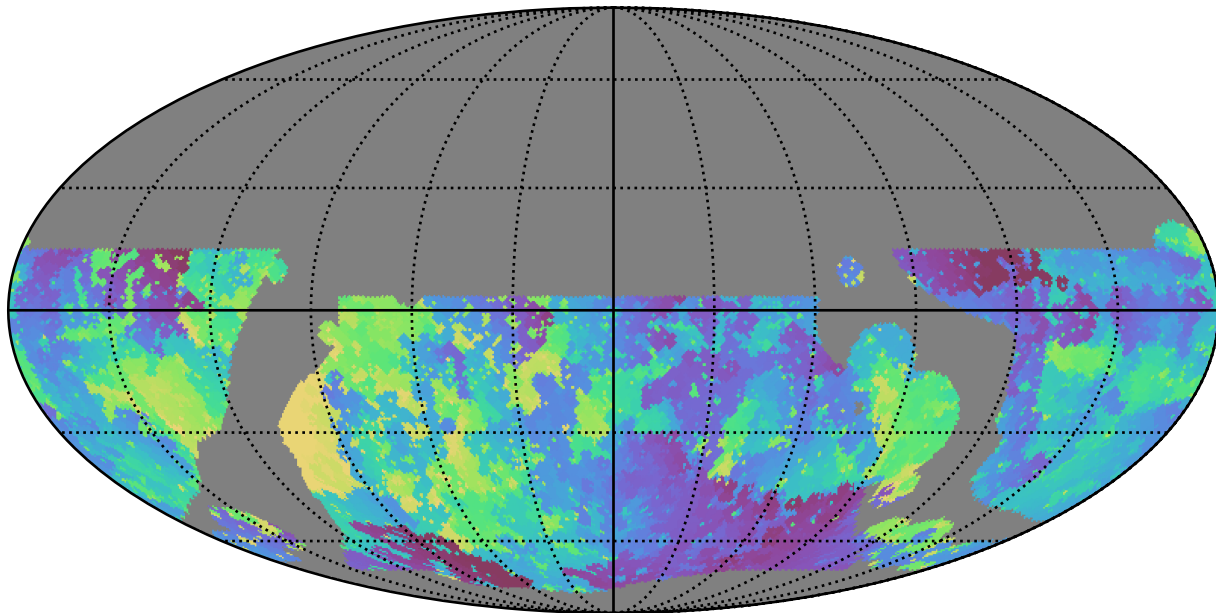
weather_cloudso0v3.5_10yrs WFD u band: Min skyBrightness
