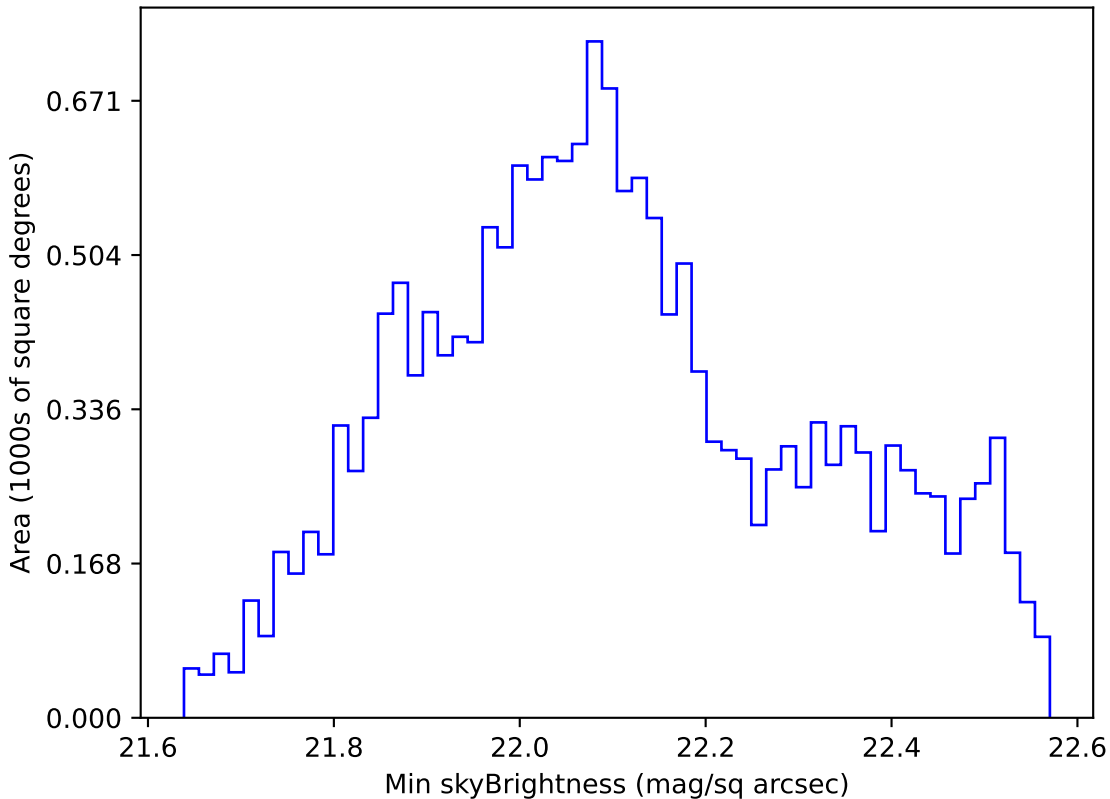
weather_cloudso0v3.5_10yrs WFD u band: Min skyBrightness
