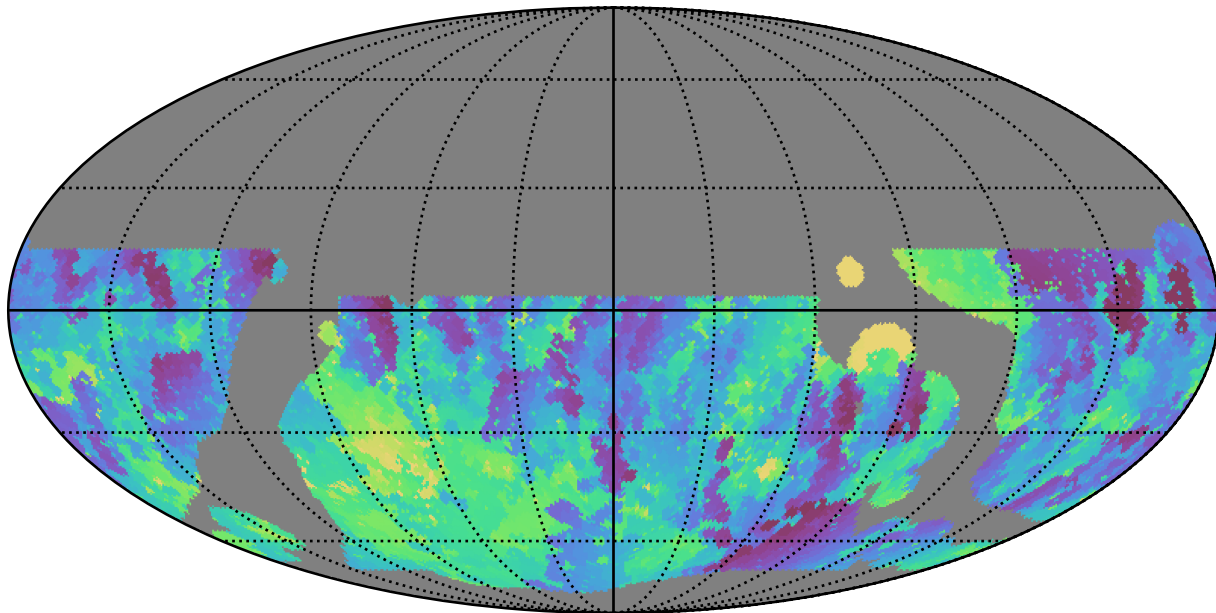
weather_cloudso0v3.5_10yrs WFD r band: Min skyBrightness
