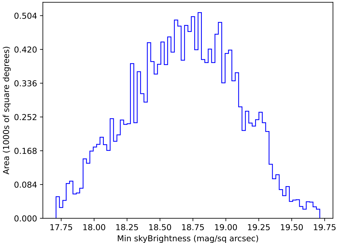
weather_cloudso0v3.5_10yrs WFD r band: Min skyBrightness
