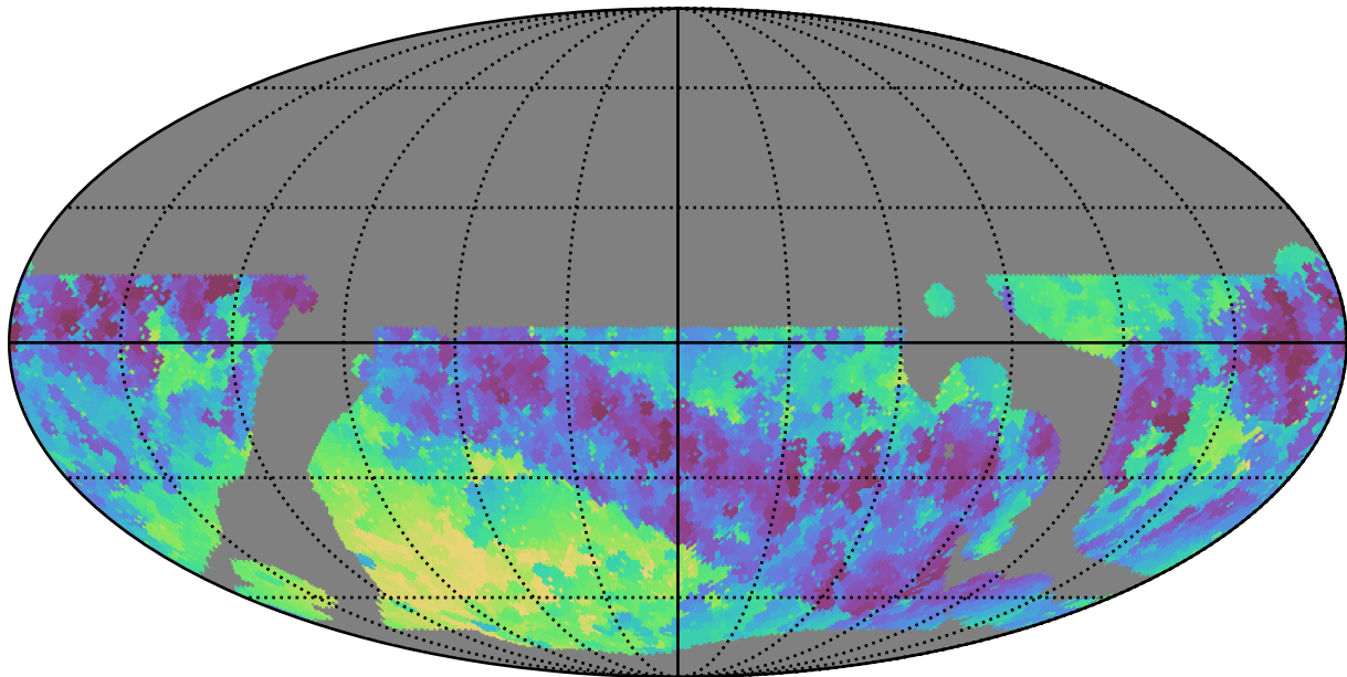
weather_cloudso0v3.5_10yrs WFD i band: Min skyBrightness
