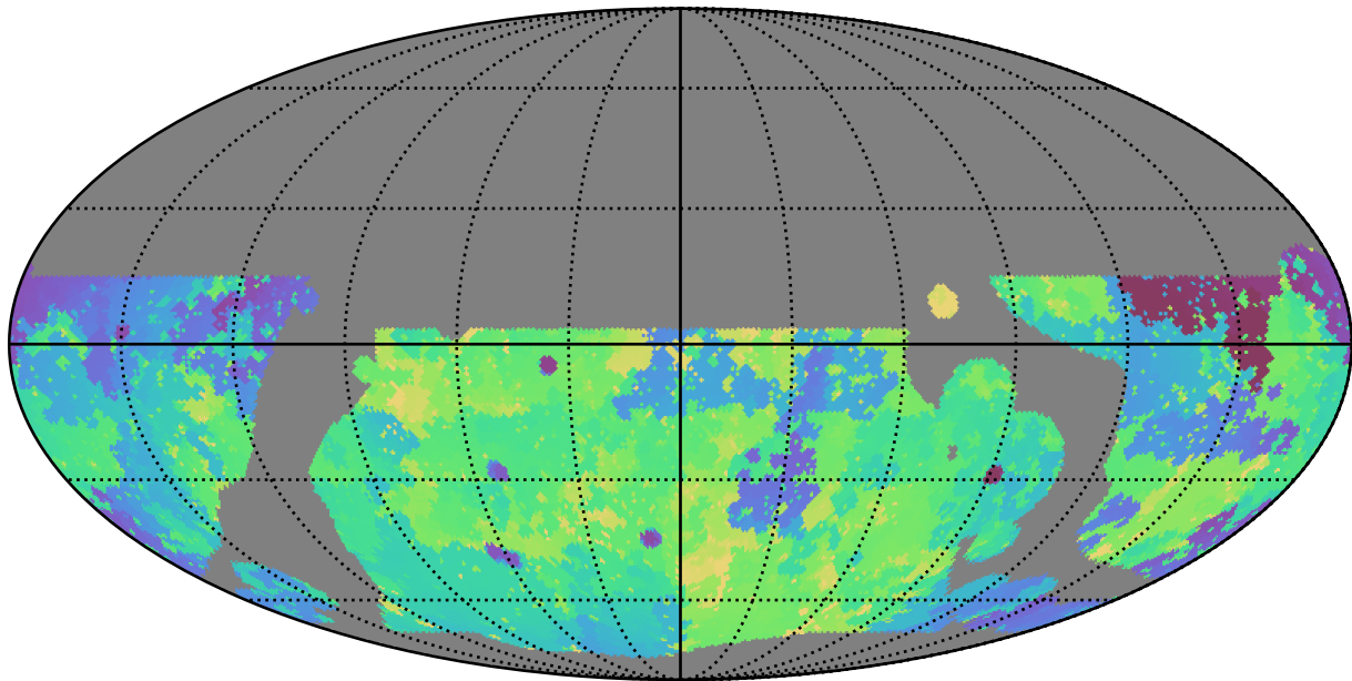
weather_cloudso0v3.5_10yrs WFD g band: Min skyBrightness
