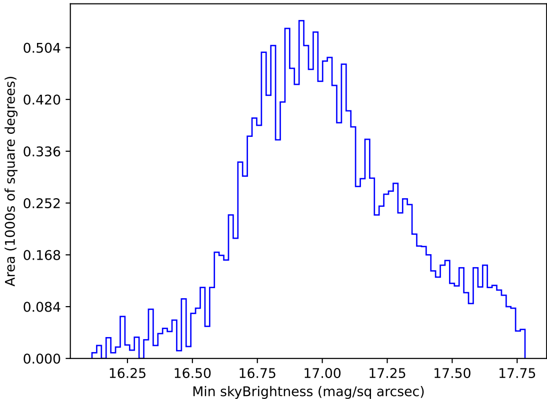
weather_cloudso0v3.5_10yrs WFD all bands: Min skyBrightness
