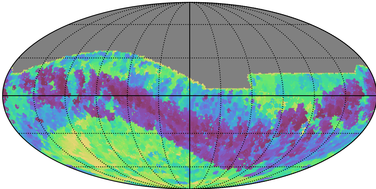
weather_cloudso0v3.5_10yrs All sky z band: Min skyBrightness
