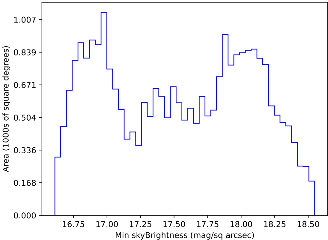
weather_cloudso0v3.5_10yrs All sky z band: Min skyBrightness
