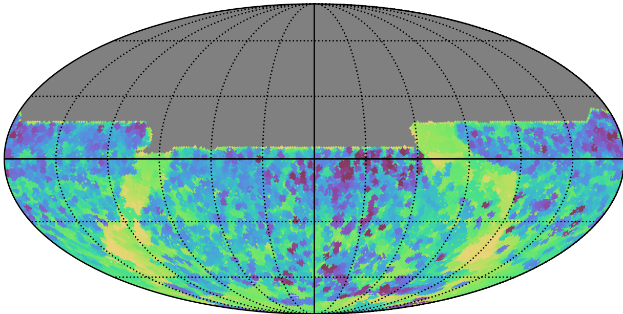
weather_cloudso0v3.5_10yrs All sky y band: Min skyBrightness
