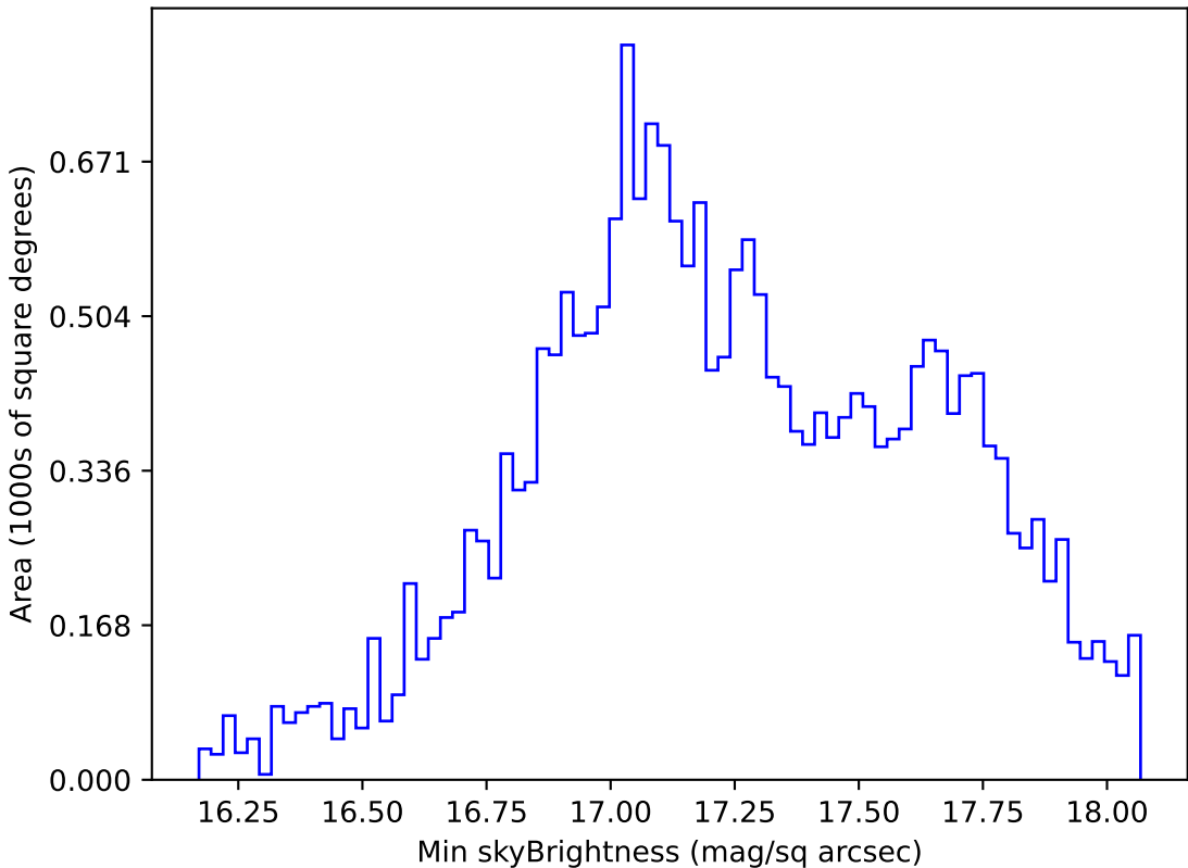
weather_cloudso0v3.5_10yrs All sky y band: Min skyBrightness
