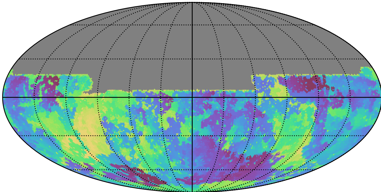
weather_cloudso0v3.5_10yrs All sky u band: Min skyBrightness
