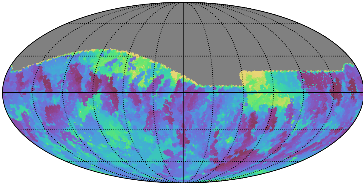
weather_cloudso0v3.5_10yrs All sky r band: Min skyBrightness
