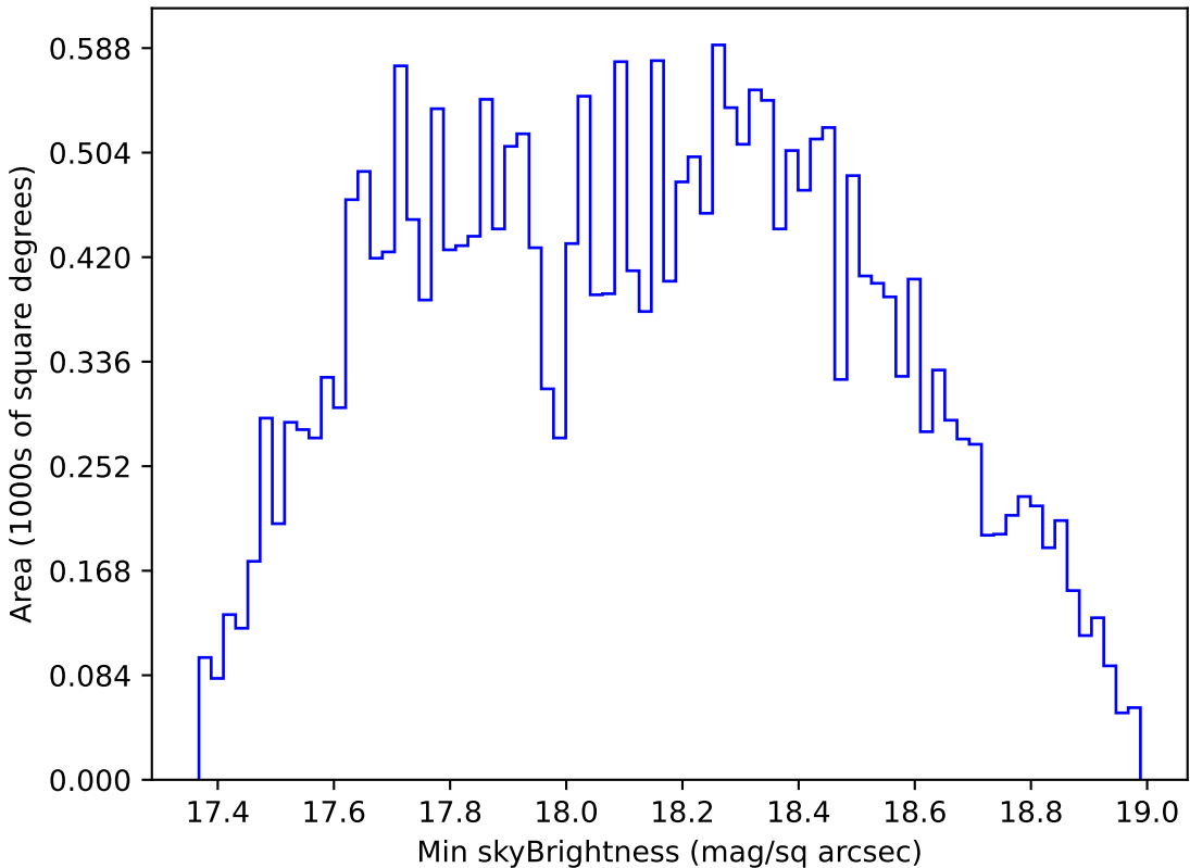
weather_cloudso0v3.5_10yrs All sky i band: Min skyBrightness
