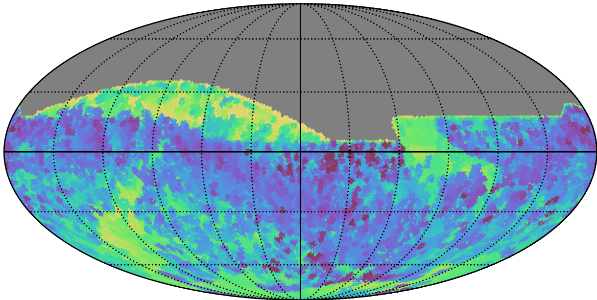
weather_cloudso0v3.5_10yrs All sky all bands: Min skyBrightness
