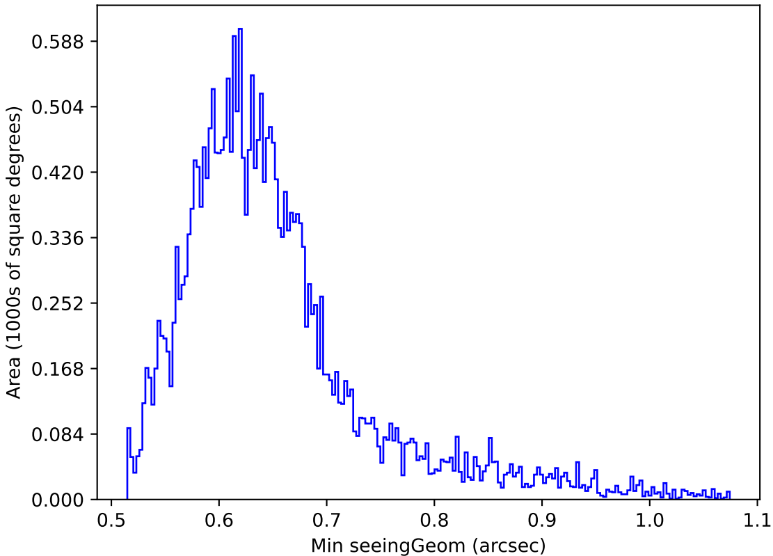
weather_cloudso0v3.5_10yrs Yr 1 z band: Min seeingGeom
