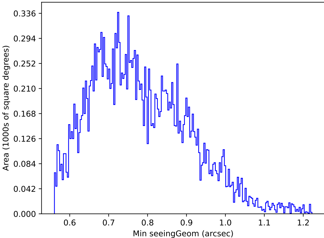
weather_cloudso0v3.5_10yrs Yr 1 u band: Min seeingGeom
