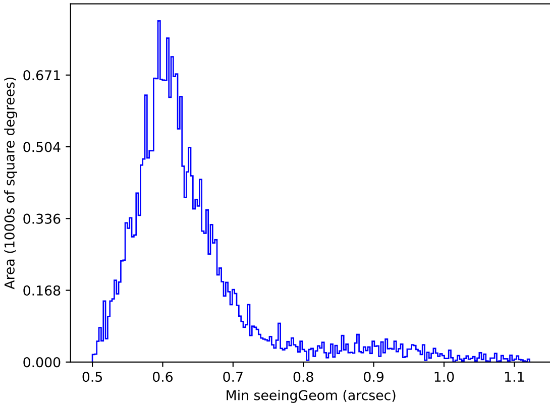
weather_cloudso0v3.5_10yrs Yr 1 r band: Min seeingGeom
