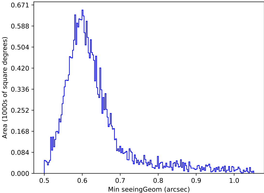
weather_cloudso0v3.5_10yrs Yr 1 i band: Min seeingGeom
