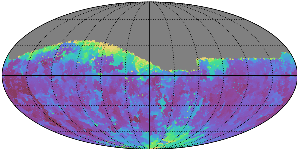
weather_cloudso0v3.5_10yrs Yr 1 g band: Min seeingGeom
