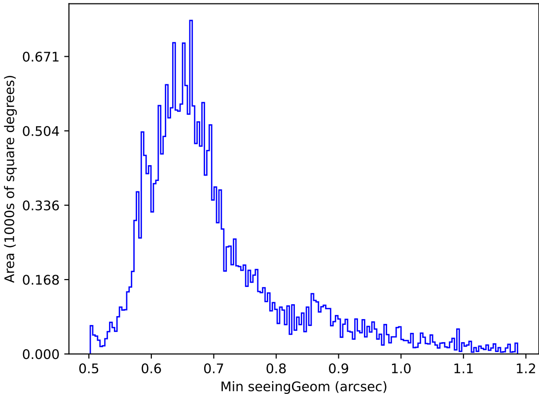
weather_cloudso0v3.5_10yrs Yr 1 g band: Min seeingGeom
