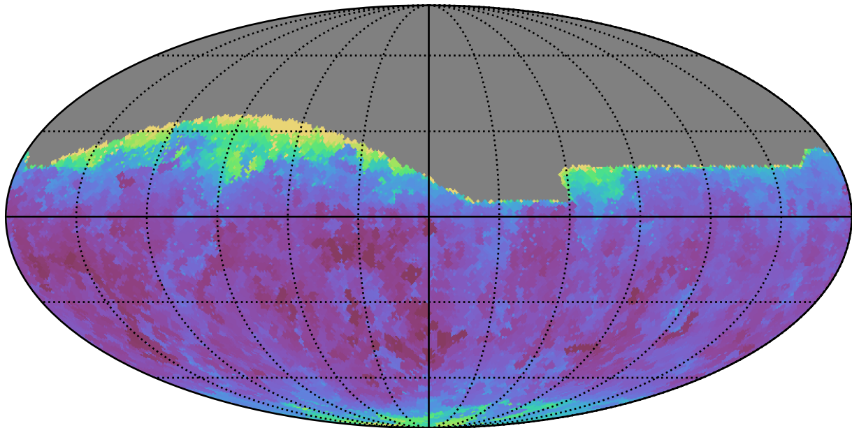
weather_cloudso0v3.5_10yrs Yr 1 all bands: Min seeingGeom
