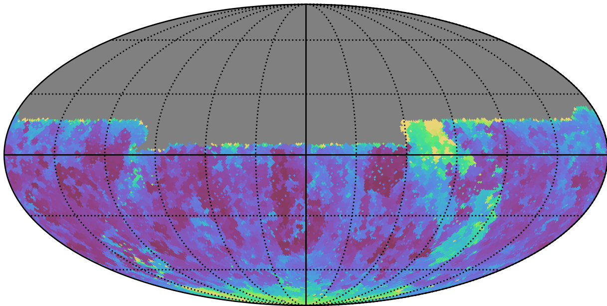
weather_cloudso0v3.5_10yrs Yr 1 y band: Min seeingEff
