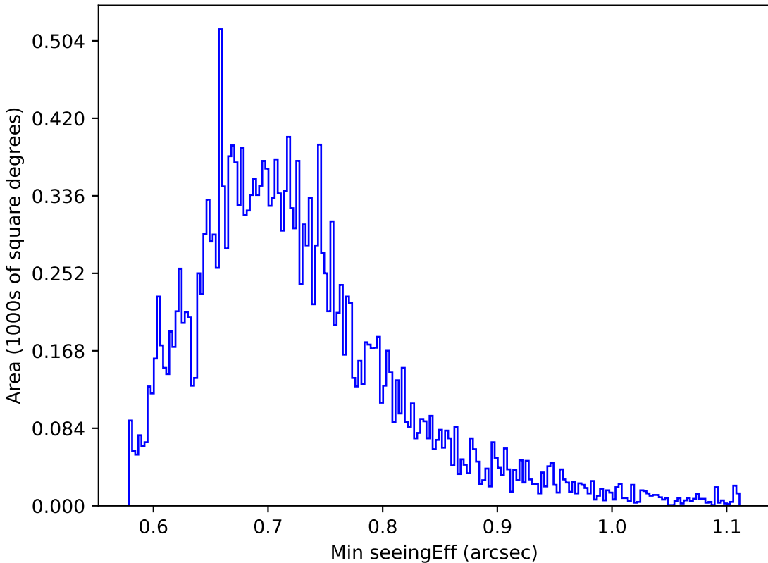
weather_cloudso0v3.5_10yrs Yr 1 y band: Min seeingEff
