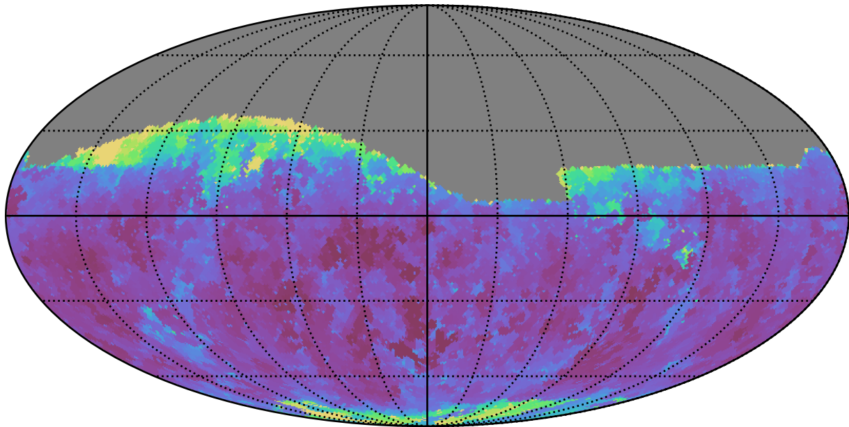
weather_cloudso0v3.5_10yrs Yr 1 i band: Min seeingEff
