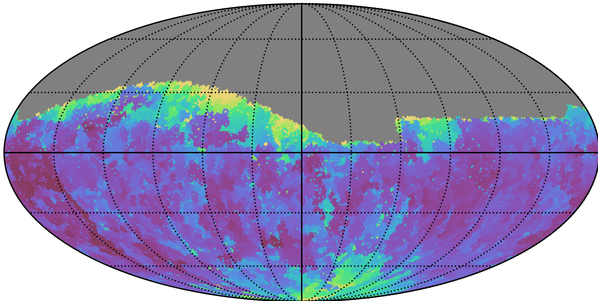
weather_cloudso0v3.5_10yrs Yr 1 g band: Min seeingEff
