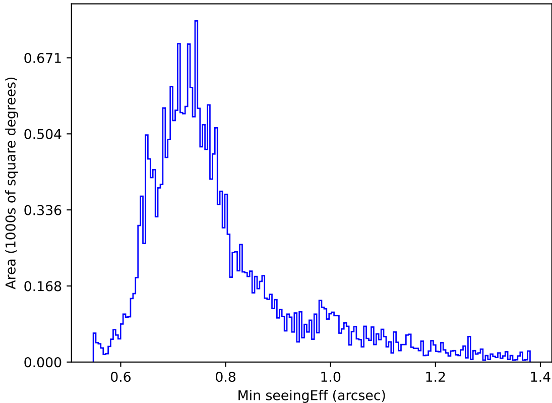
weather_cloudso0v3.5_10yrs Yr 1 g band: Min seeingEff
