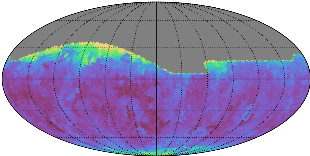
weather_cloudso0v3.5_10yrs Yr 1 all bands: Min seeingEff
