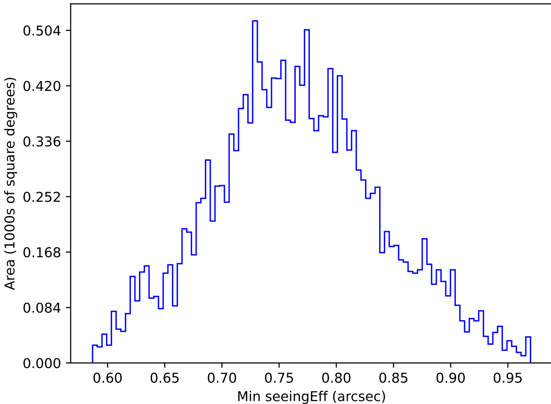
weather_cloudso0v3.5_10yrs WFD u band: Min seeingEff
